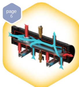
Distribution low loss header - SKE
